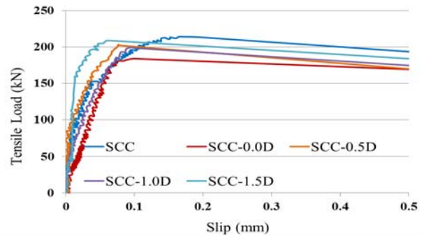
Fig. 9 Load – Slip Relationship for SCC
