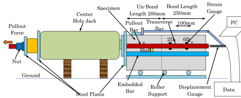
Fig. 7 Experimental setup and Specimen Detail
