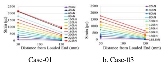
Case-01 b. Case-03 Fig. 16 Strain Profile of NC Specimens
