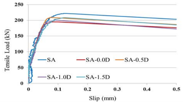
Fig. 10 Load – Slip Relationship for SA
