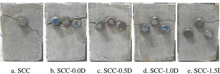
Fig. 14 Fracture Pattern of SCC
