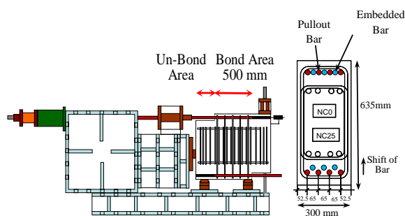
Fig. 2 Experimental Setup and Detail [2]
