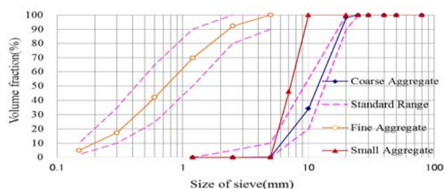
Fig. 4 Gradation of Aggregate for NC and SCC
