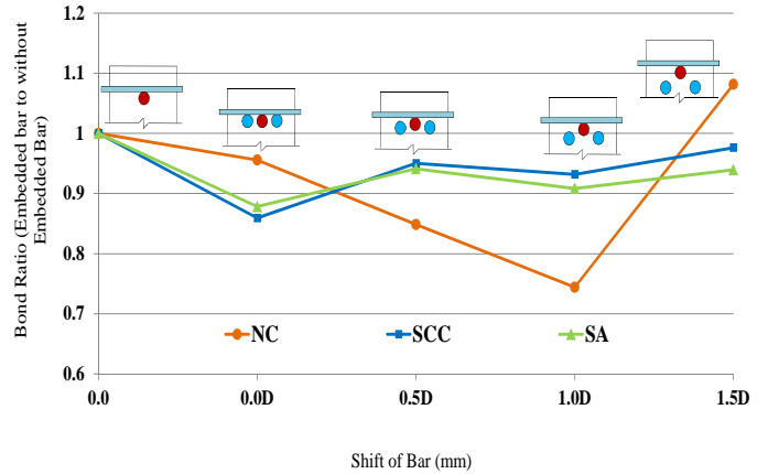
Fig. 12 Relationship between Bond Ratio-Shift of Bar
