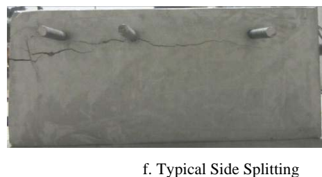
f. Typical Side Splitting
