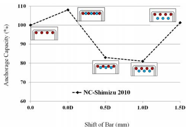
Fig. 3 Relationship between Anchorage Capacity-Shift of Bar
