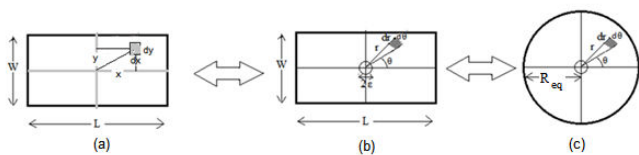
Fig. 1 The rectangular field with dimension W \times L cm 2 (in Cartesian coordinates (a) and in polar coordinates (b)) is equivalent to a circular field with radius R_{eq} cm (c) on a plane at SSD=100cm
