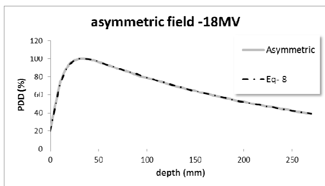
Fig. 5 The PDD measured for an asymmetric rectangular field (5, 5×2, 8) (gray line) and its calculated equivalent square 8×8 (dash-dot) for 18MV energies with relative error 0.6±0.9%
