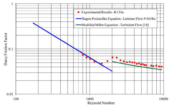
Fig. 6 Darcy friction factor variation with Reynolds number for R134a
