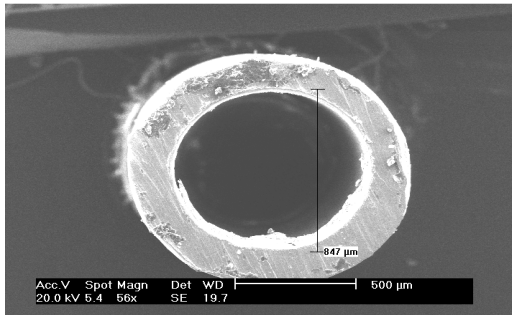
Fig. 4 SEM image of tested micro-tube
