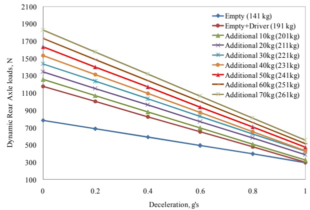
Fig. 3 Dynamic rear axle loads for unladen and various pillion loads
