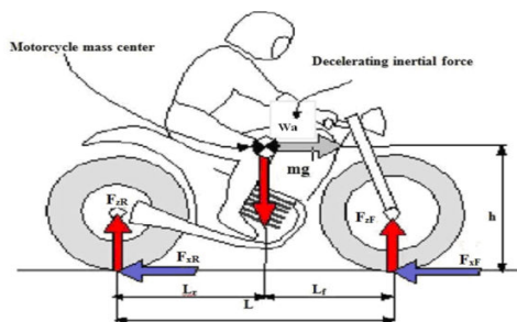
Fig. 2 Load transfer effect during braking
