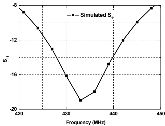
Fig. 5 Simulated input return loss ( S_{11} )
