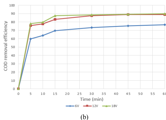
Fig. 3 Efficiency of electrocoagulation process for COD removal by iron electrode (a) initial pH 4 (b) initial pH 9
