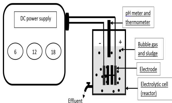
Fig. 1 Diagram of experiment setup for electrocoagulation process
