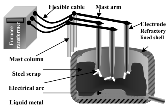
Fig. 1 Typical electrical arc furnace
