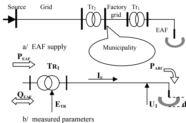
Fig. 3 Studied model
