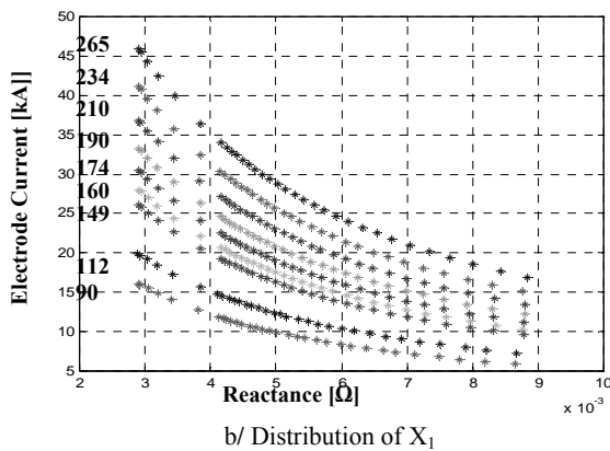
Fig. 5 Calculation of Z_1 form the 9x32 measurements
