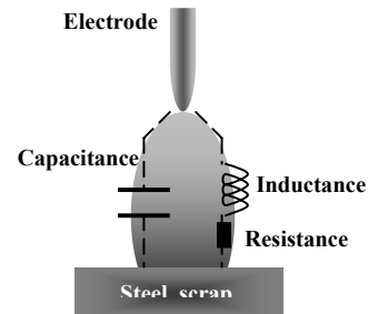
Fig. 6 Electric arc model
