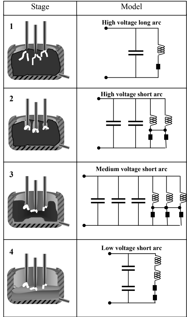
Fig. 8 The proposed model of EAF for each melting stage
