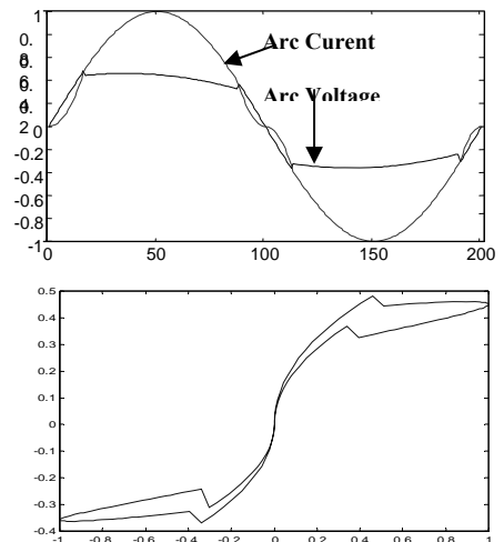
Fig. 9 Temporal and [IV] representation of electric arc current & voltage
