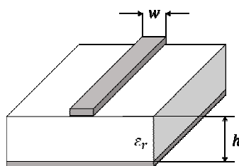
Fig. 1 Microstrip Transmission Line
