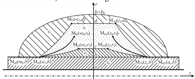
Fig. 6 Modelled cable joint by using five - layer dielectric system and very thin deflector's cones, having polynomial form.
