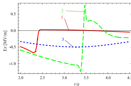
Fig. 11 Axial component of electric field distribution, E_z (MV/m), in radial direction, r/a for z/a = 0.5 (curve 1), z/a = 2.0 (curve 2), z/a = 10.0 (curve 3)
