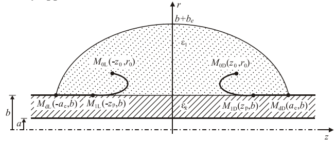
Fig. 3 Geometrically modelled cable joint
