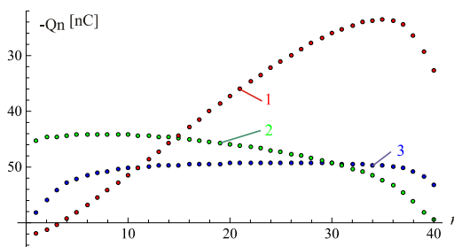
Fig. 10 Charge distribution at outer conductor (1), dielectrics boundary (2) and deflector (3)
