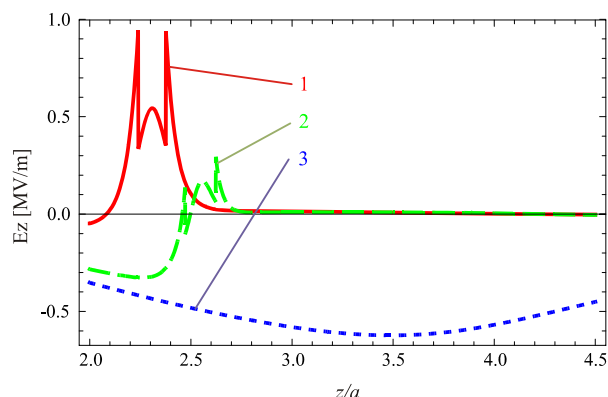
Fig. 19 Axial component of electric field distribution in axial direction, for different distance from z axis
