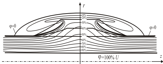
Fig. 7 Equipotential curves at modelled cable joint by using five-layer dielectric system and very thin deflector's cones
