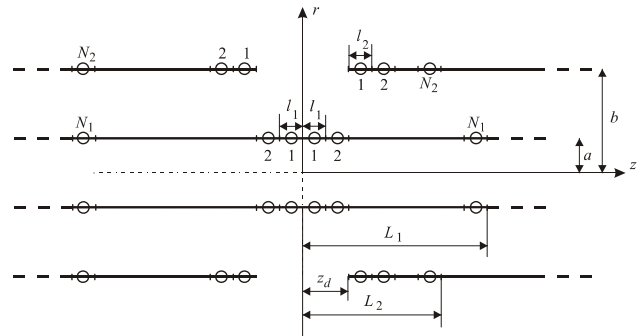
Fig. 1 Non-modeled cable joint
