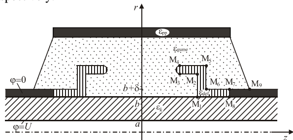
Fig. 9 Refractive modelled cable joint
