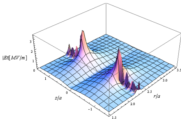
Fig. 2 Tangential component ( E_t ) of electrical field distribution
