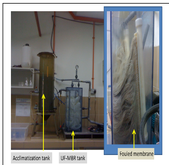
Fig. 1 The overview of the membrane bioreactor during the start-up process
