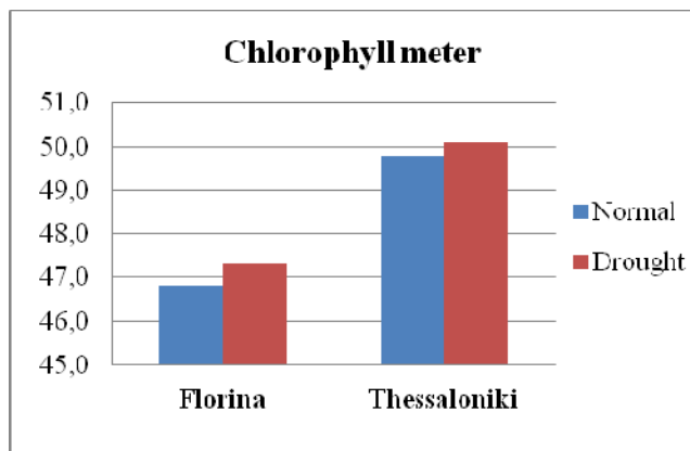
Fig. 6 Chlorophyll meter readings (SPAD) at two locations (Florina and Thessaloniki) and two treatments, foul water (normal) and 60% water (drought)
