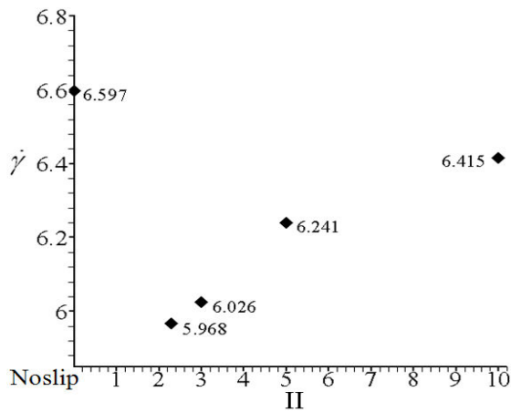
Fig. 6 The peak of \dot{\gamma} versus II_{crit} on bottom down-stream wall of Newtonian fluid at \alpha = 0.1
