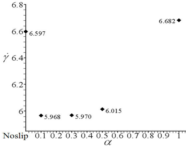
Fig. 5 The peak of \dot{\gamma} versus \alpha on bottom downstream wall of Newtonian fluid at II = 2.3
