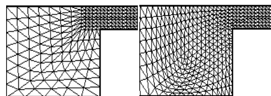
(a) mesh1
