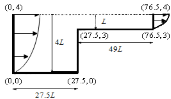
Fig. 1 Schematic of 4:1 contraction flow
