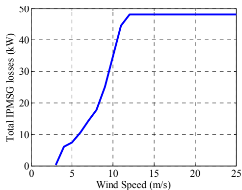
Fig. 6 Total losses for the IPMSG
