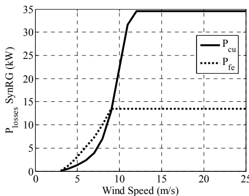
Fig. 8 Copper and iron losses for the SynRG
