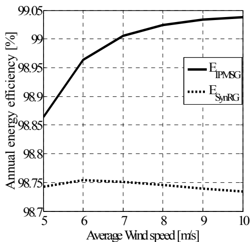
Fig. 11 Annual energy efficiency of the generators
