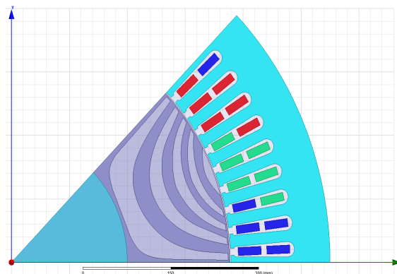
Fig. 7 Cross-section of the SynRM
