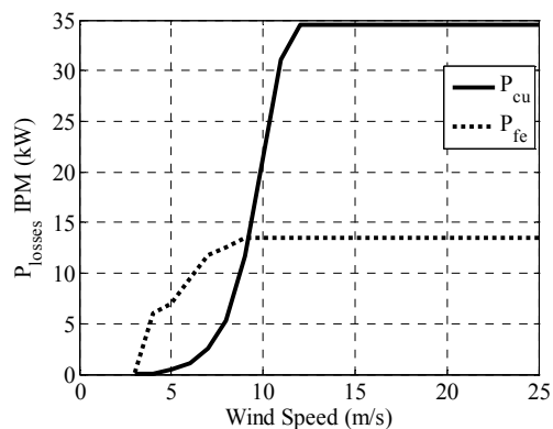
Fig. 5 Copper and iron losses for the IPMSG
