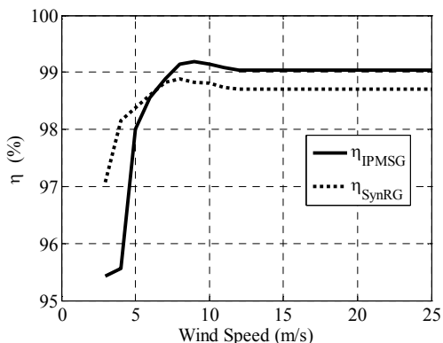
Fig. 10 Machine efficiency
