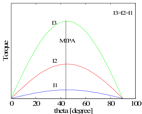
Fig. 1 Operation diagram for SynRM with constant current
