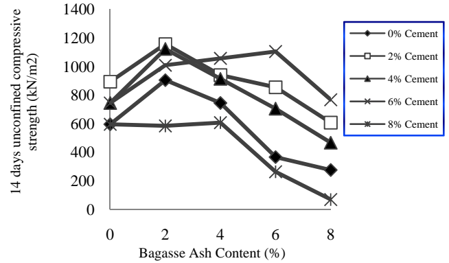
Fig. 12 Variation of unconfined compressive strength (14 days curing) with bagasse ash content for soil-cement-bagasse ash mixtures (Modified Proctor compaction)
