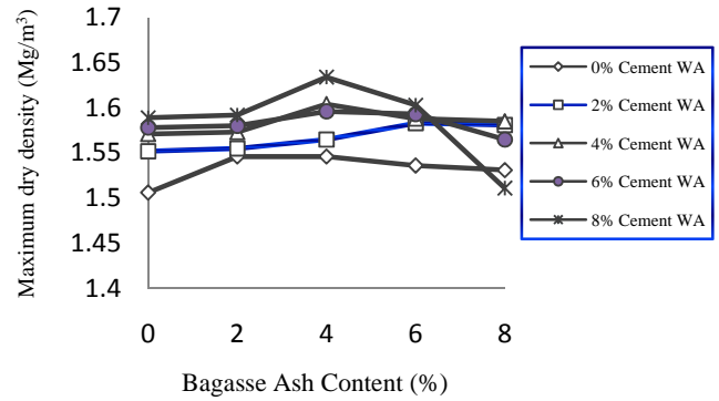
Fig. 2 Variation of maximum dry density for with bagasse ash content for soil-cement-bagasse ash mixtures (West African Standard compaction)
