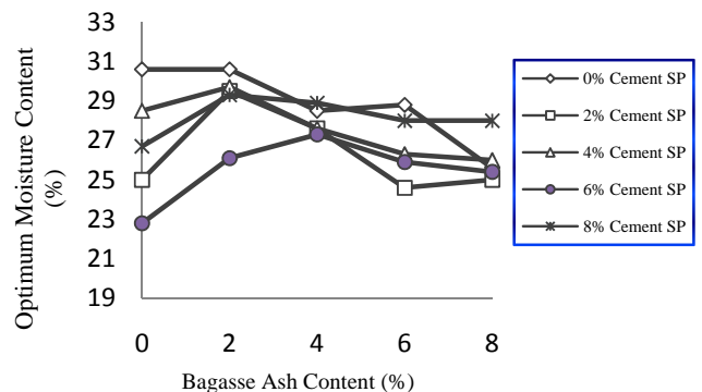
Fig. 4 Variation of optimum moisture content with bagasse ash content for soil-cement-bagasse ash mixtures (Standard Proctor compaction)
