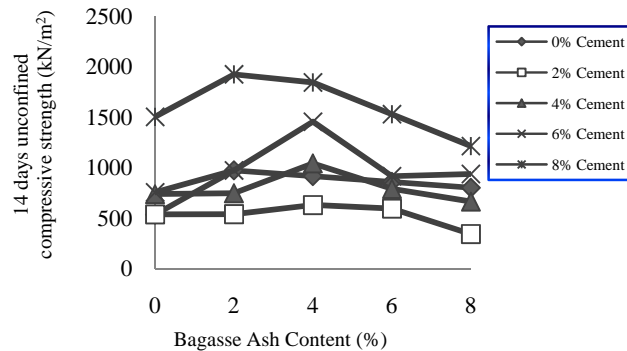
Fig. 11 Variation of unconfined compressive strength (14 days curing) with bagasse ash content for soil-cement-bagasse ash mixtures (West African Standard compaction)
