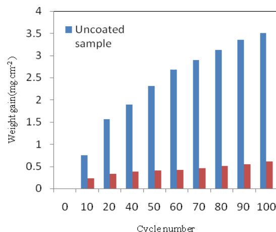
Fig. 4 Specific weight gain as a function of cycle number after cyclic oxidation
