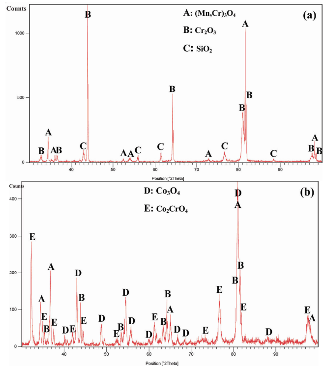
Fig. 3 XRD pattern of (a) uncoated and (b) coated specimens after 200h isothermal oxidation at 800°C
