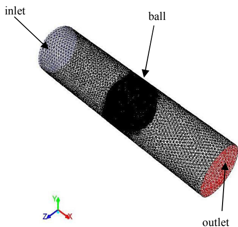
Fig. 4 Numerical calculations mesh
