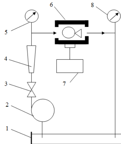
Fig. 2 Experimental setup
