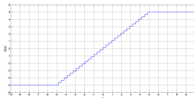
Fig. 3 Q-function of the uniform quantizer
