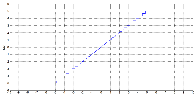
Fig. 4 Q-function of the floating point non-uniform quantizer
