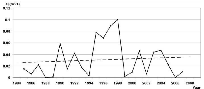
Fig. 14 Multiannual variation of annual minimum at Codaesti hydrometric station, river Dobrovat and tendency of these variations
