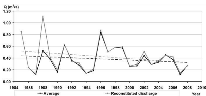
Fig. 4 Multi-annual variation of mean annual flow measured and reconstituted at Codaesti hydrometric station, river and Dobrovat tributary
