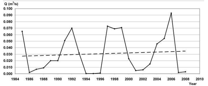
Fig. 12 Multiannual variation and minimal annual flow rates at Solesti hydrometric station Solesti, river Vaslui and its tributaries
