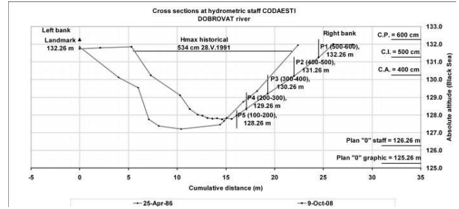
Fig. 16 Hydrometric transverse profile of the Codaesti (on Dobrovat River) after producing the historic peak of 28.V.1991
