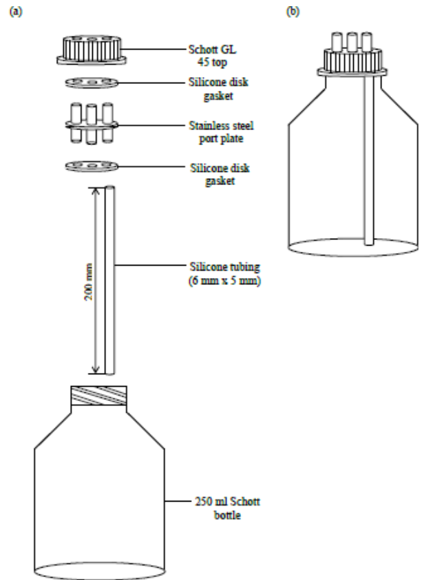
Fig. 3 (a) Assembly and (b) assembled collection bottles
