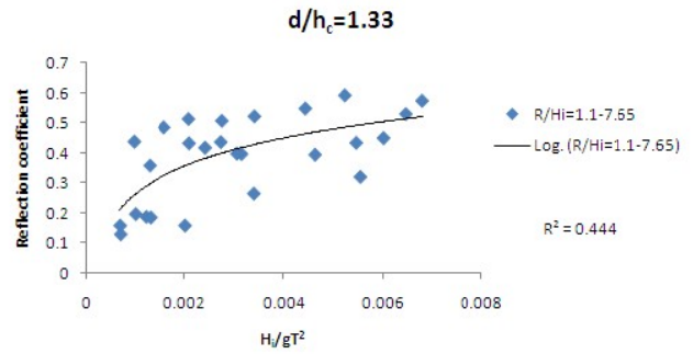
Fig. 6 Variation of K_r with H_i/gT^2 for R/H_i=1.1-7.65
