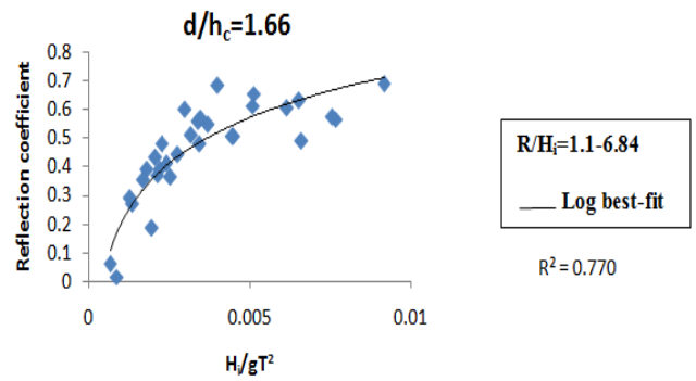
Fig. 14 Variation of K_r with H_i/gT^2 for R/H_i=1.1-6.84
