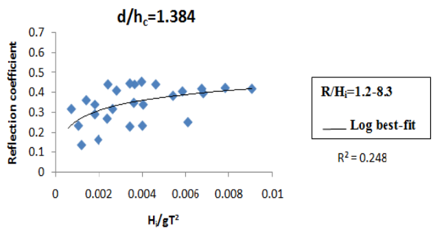
Fig. 9 Variation of K_r with H_i/gT^2 for R/H_i=1.2-8.3
