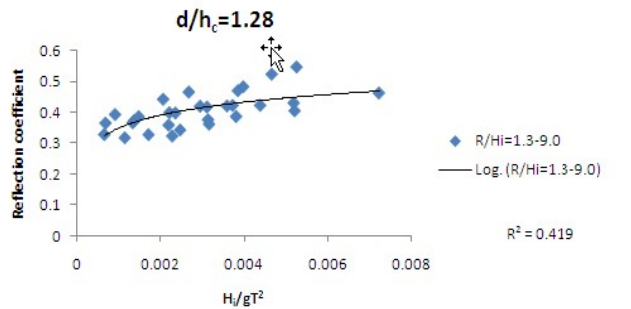
Fig. 8 Variation of K_r with H_i/gT^2 for R/H_i=1.3-9.0
