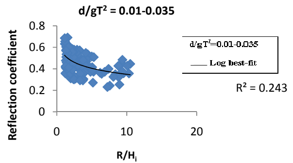
Fig. 15 Variation of K_r with R/H_i for d/gT^2=0.01-0.035
