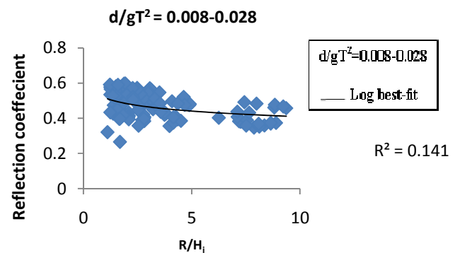
Fig. 17 Variation of K_r with R/H_i for d/gT^2=0.008-0.028
