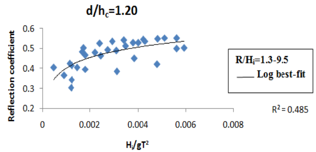
Fig. 7 Variation of K_r with H_i/gT^2 for R/H_i=1.3-9.5
