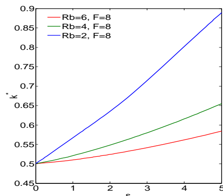
Fig. 13. Graph showing the relationship between the most unstable mode k^* and the arc-length s for a viscoelastic liquid jet, where the dimensionless numbers are Re = 1000 , We = 10 , De = 15 , \alpha = 20 .
