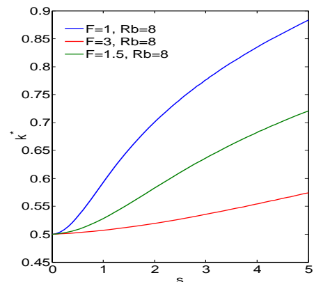
Fig. 10. Graph showing the relationship between the most unstable mode k^* and the arc-length s for a viscoelastic liquid jet, where the dimensionless numbers are Re = 1000, We = 10, De = 15, \alpha = 20 .
