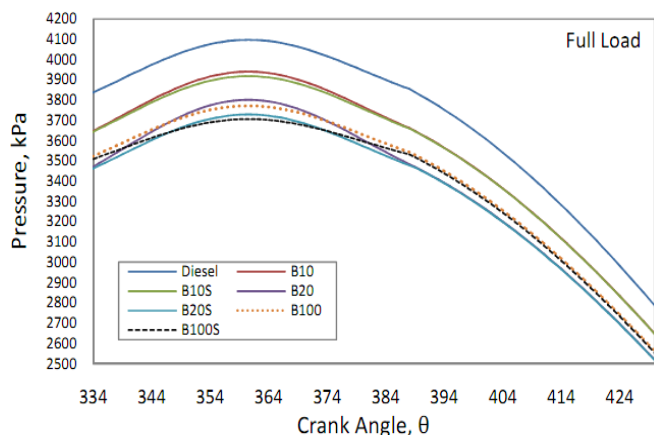
Fig. 2 Pressure versus crank angle for biodiesel-diesel blends
