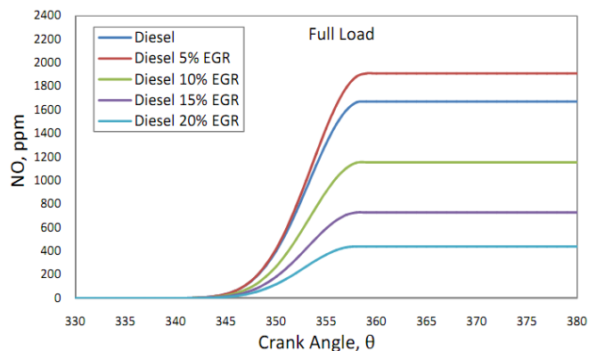
Fig. 9 Nitric oxide emissions versus crank angle with fuel diesel with different EGR rates
