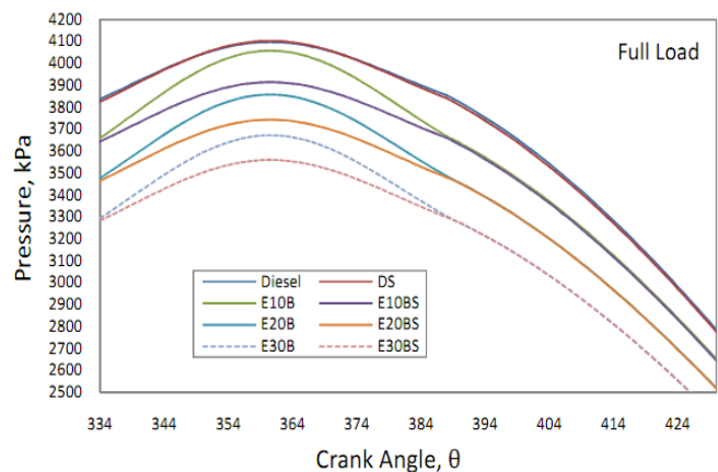
Fig. 1 Pressure versus crank angle for ethanol-diesel blends
