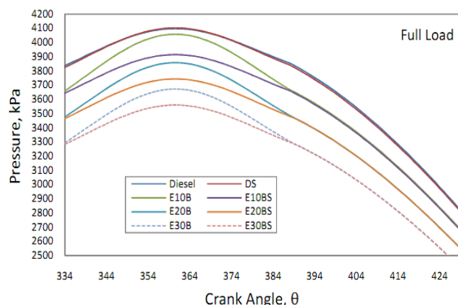
Fig. 1 Pressure versus crank angle for ethanol-diesel blends
