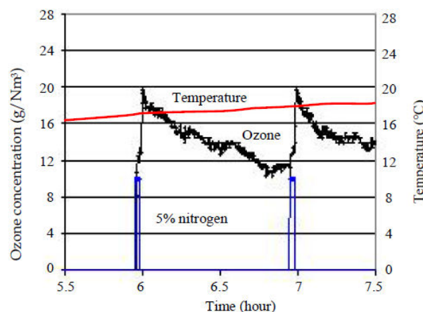
Fig. 15 5% Nitrogen addition without rotation
