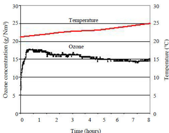
Fig. 8 The ozone concentration (New electrode)
