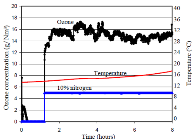
Fig. 10 Ozone zero phenomena
