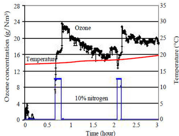
Fig. 14 10% Nitrogen addition during 600rpm operation
