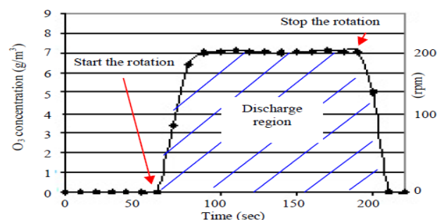
Fig. 7 Variation of ozone concentration for different rotation mode maximum rotating speed is 200 rpm
