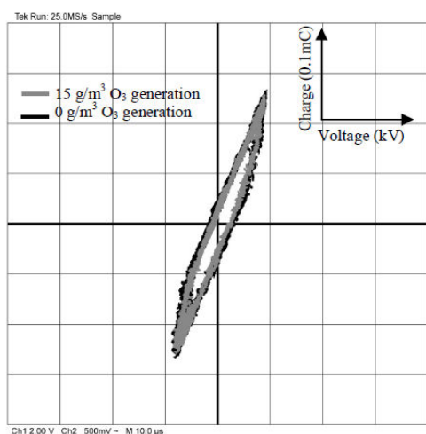
Fig. 12 Lissajous figure during zero ozone production and after mixing gas (15g/m³)
