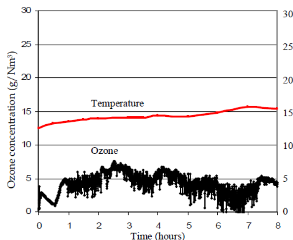
Fig. 9 Ozone concentration after few days experiments
