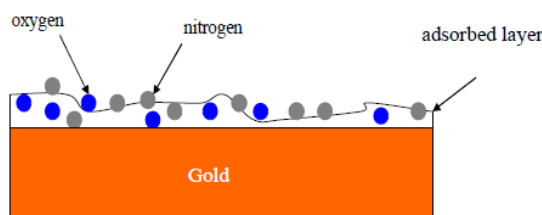
Fig. 13 Schematic surface electrode
