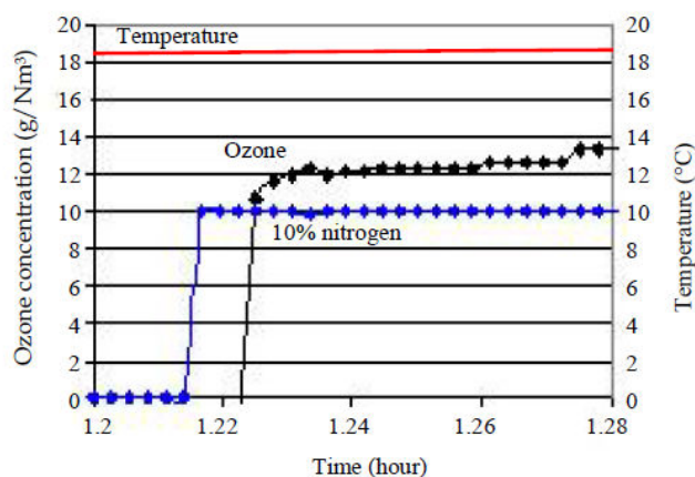
Fig. 11 Expanded addition 10% nitrogen during 600rpm operation
