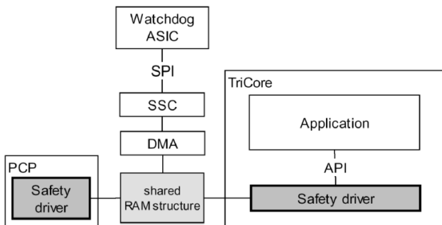
Fig. 3 External safety monitor
