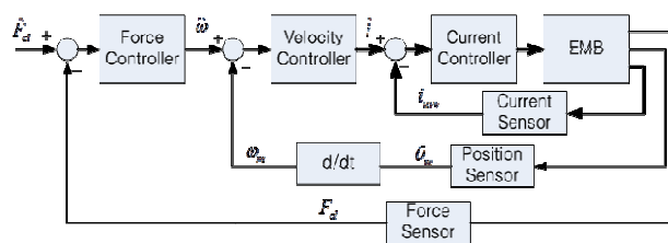
Fig. 4 Block diagram of EMB control system
