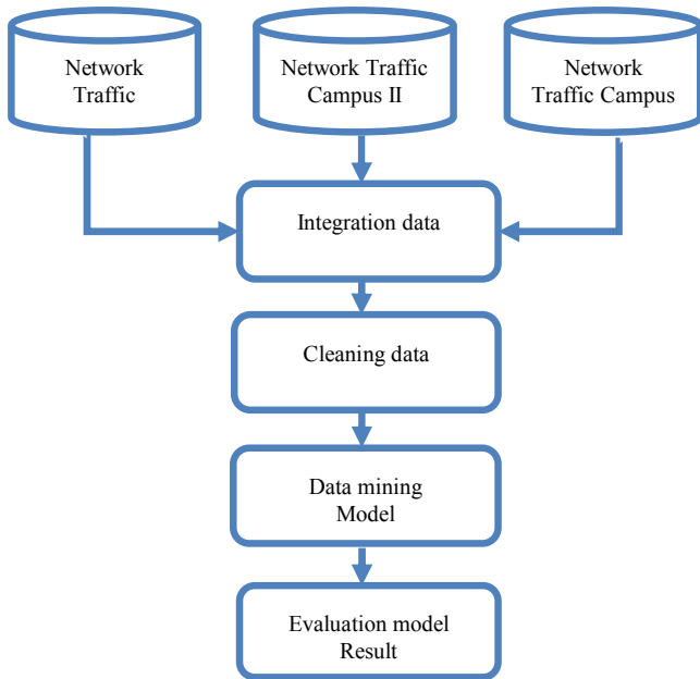
Fig. 1 Framework for network traffic prediction method
