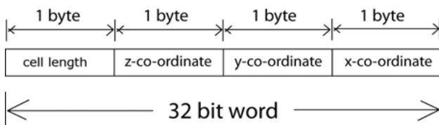
Fig. 8 Leaf node vertex structure
