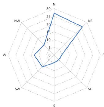
Fig. 29 Wind rose at 18 m above the ground for the month of November
