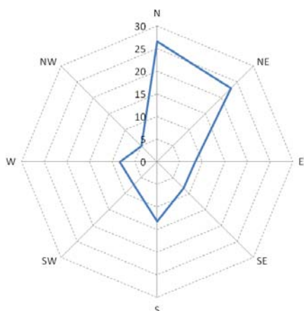
Fig. 20 Wind rose at 18 m above the ground for the month of February
