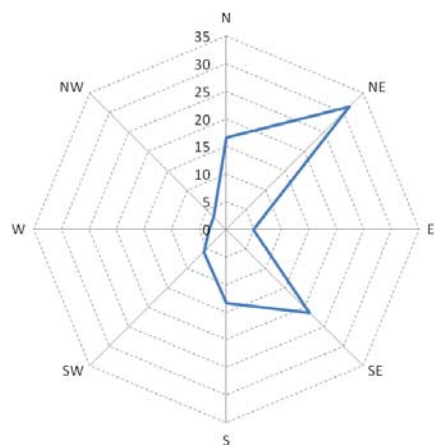
Fig. 27 Wind rose at 18 m above the ground for the month of September
