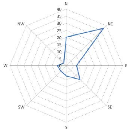
Fig. 28 Wind rose at 18 m above the ground for the month of October
