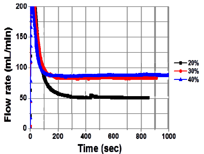
Fig. 8 The effects of rpm on flow rate
