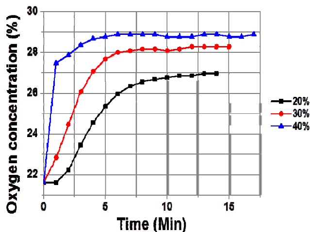
Fig. 9 The effects of rpm on oxygen concentration
