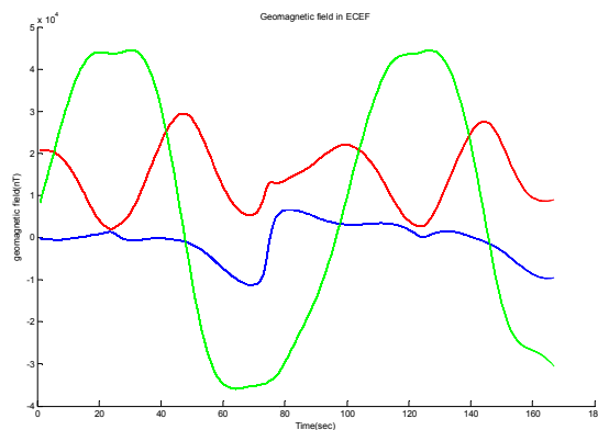
Fig. 14 Geomagnetic Field Estimation in ECEF
