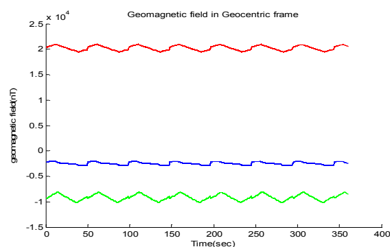
Fig. 13 Geomagnetic Field Estimation in Geocentric Frame
