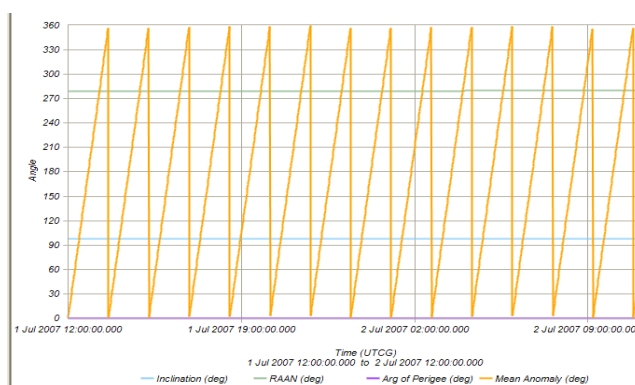
Fig. 4 Keplerian Elements from STK
