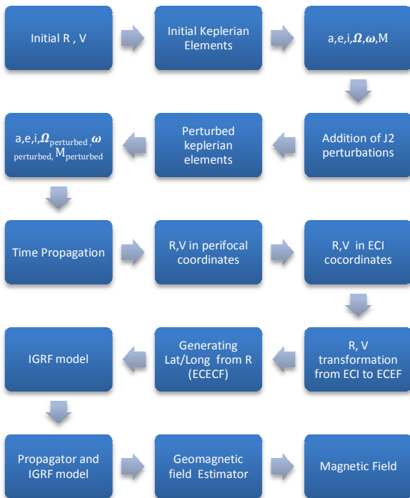
Fig. 16 Flow Diagram
