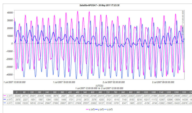
Fig. 15 Geomagnetic Field Estimation in ECEF from STK
