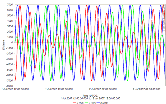
Fig. 12 Position Vector in ECEF Frame from STK
