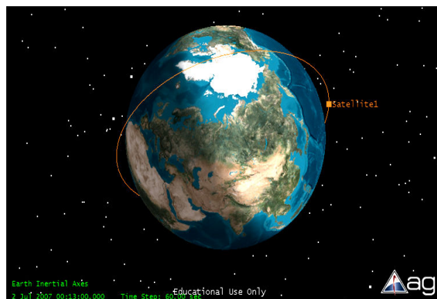
Fig. 1 ICUBE-1 Orbit in STK
