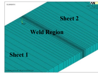
Fig. 8 Finite element mesh
