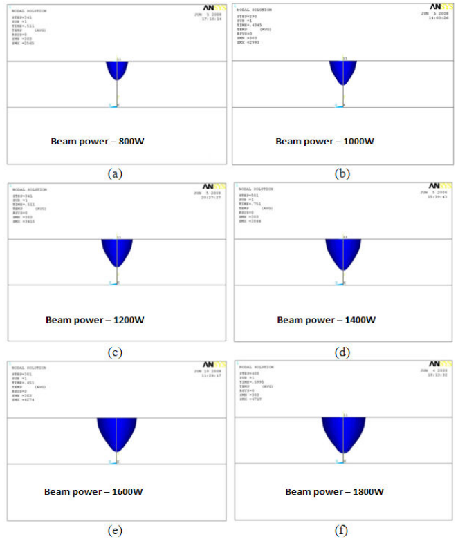
Fig. 12 (a)-(f) The effect of beam power on the bead geometry for the laser parameters: 800mm/min WS and 85^{\circ} BA
