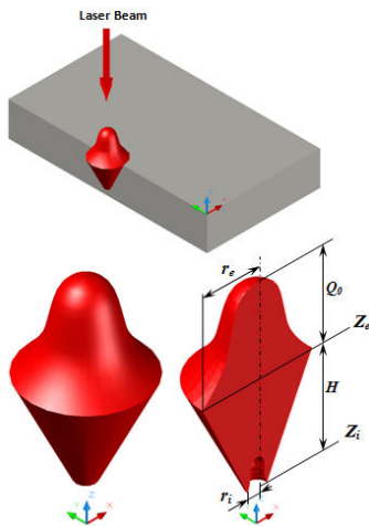
Fig. 7 Schematic of 3D Conical Heat source model
