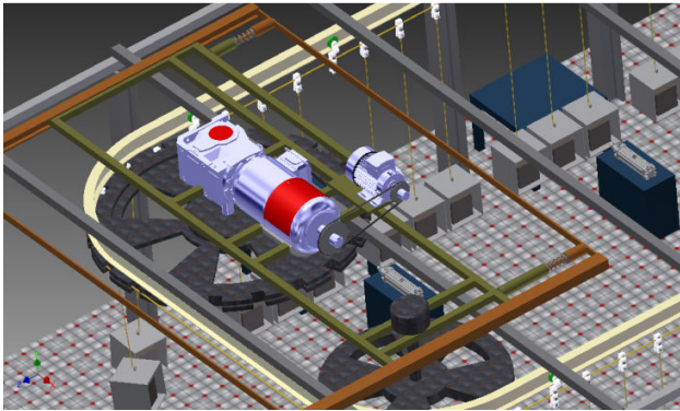
Fig. 3 Drive unit
