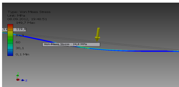
Fig. 6 Breakpoint of the rope
