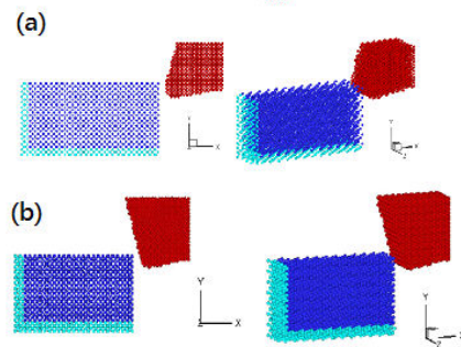
Fig. 2 Diagram of initial conditions of different simulation examples (a) Round edge diamond cutter with nose radius of 5\text{\AA} , rake angle of 15^\circ (b) Round edge diamond cutter with nose radius of 5\text{\AA} , rake angle of -15^\circ
