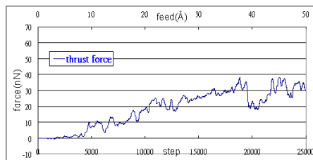
(b) Thrust force
