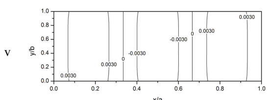
(e) \Omega/\omega_1=5.4108
