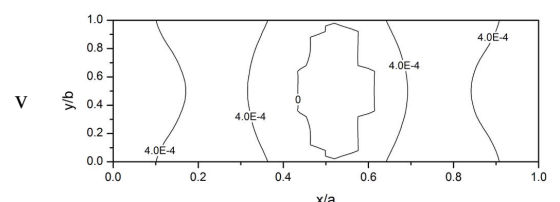
(f) \Omega/\omega_1=7.1456
