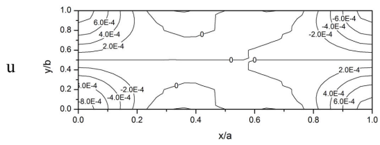
(c) \Omega/\omega_1=3.0749
