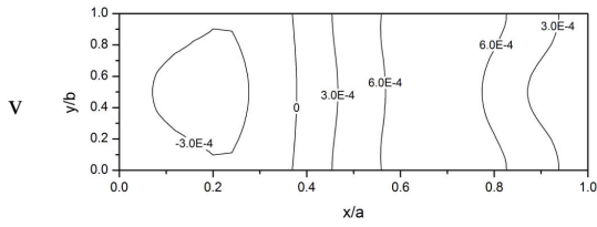
(c) \Omega/\omega_1=3.0749
