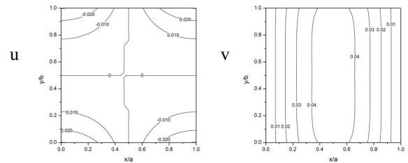
(b) \Omega/\omega_1 = 1.0
