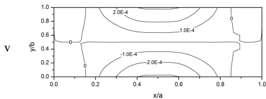
(e) \Omega/\omega_1=5.4108
