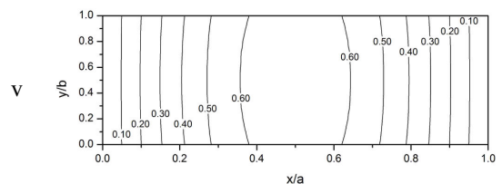
(b) \Omega/\omega_1=0.9999
