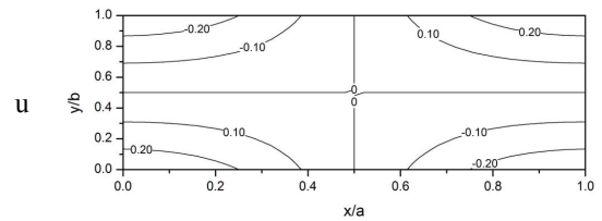
(a) \Omega/\omega_1=0
