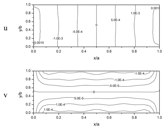
(a) \Omega/\omega_1=0
