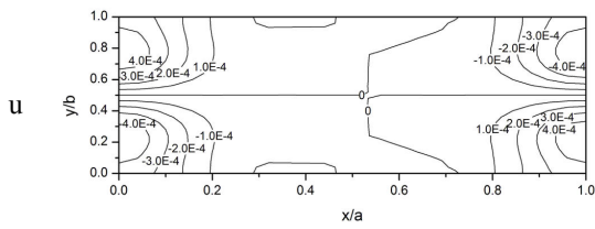
(c) \Omega/\omega_1=3.0749
