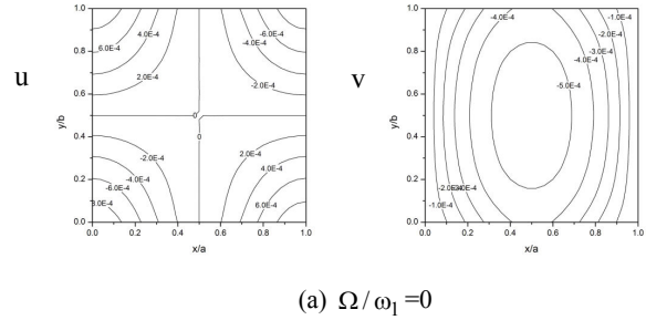
Fig 7 The forced response plots of an axially moving plate subjected to linearly, anti-symmetrically distributed excitations a/b = 3, \tilde{\nu} = 0.01, \tilde{c} = 0.1
