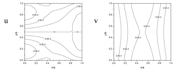
(c) \Omega/\omega_1 = 1.321
