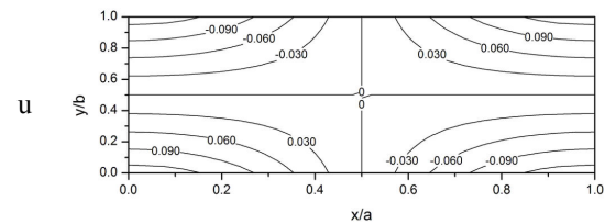
(a) \Omega/\omega_1=0
