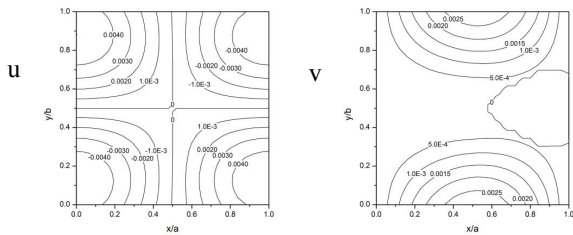
(f) \Omega/\omega_1 = 2.3901
