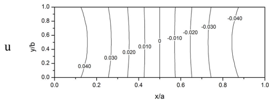
(c) \Omega/\omega_1=3.0749
