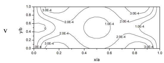
(f) \Omega/\omega_1=7.1456
