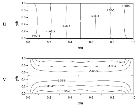
(b) \Omega/\omega_1=0.9999
