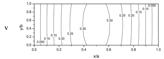
(b) \Omega/\omega_1=0.9999
