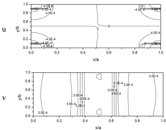
(e) \Omega/\omega_1 = 5.2899
