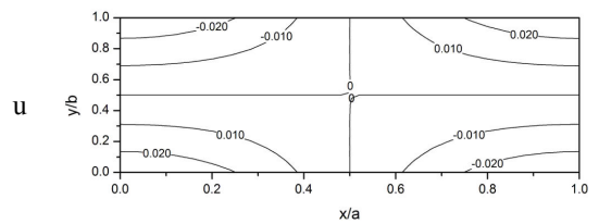
(a) \Omega/\omega_1=0
