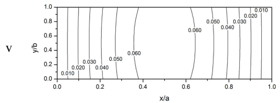
(b) \Omega/\omega_1=0.9992
