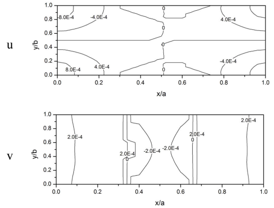
(f) \Omega/\omega_1 = 6.8650
