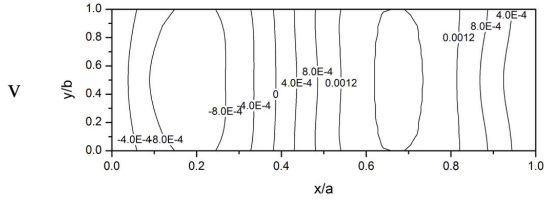
(c) \Omega/\omega_1=3.0749
