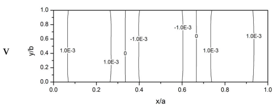
(e) \Omega/\omega_1=5.4108
