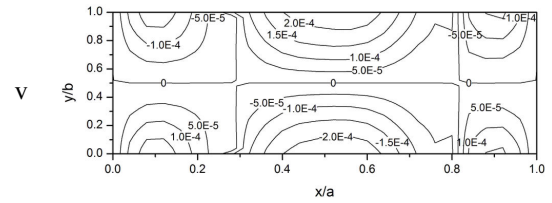
(f) \Omega/\omega_1=7.1456
