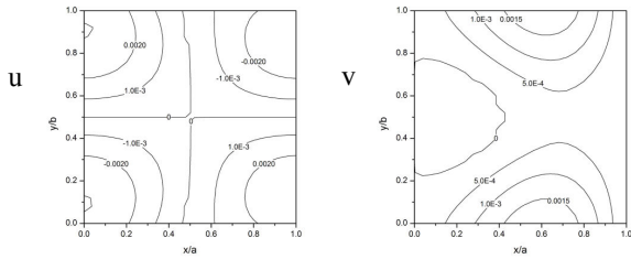
(e) \Omega/\omega_1 = 2.3079
