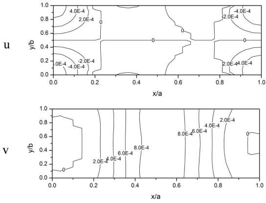
(c) \Omega/\omega_1 = 3.0529
