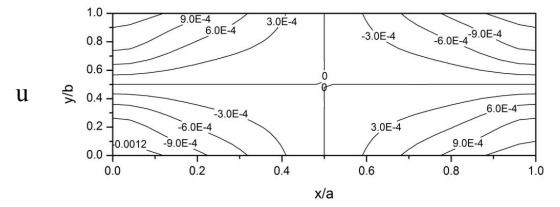
Fig. 5 The forced response plots of an axially moving plate subjected to linearly, anti-symmetrically distributed excitations a/b=3, \tilde{V}=0.01, \tilde{c}=0.01
