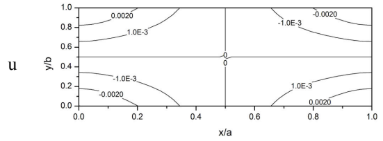
Fig. 6 The forced response plots of an axially moving plate subjected to excitations linearly, anti-symmetrically distributed on the middle halves of the edges a/b=3, \tilde{V}=0.01, \tilde{c}=0.01
