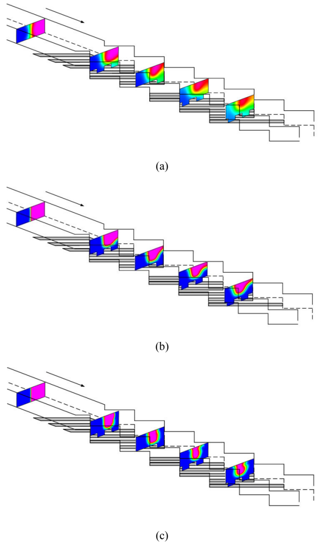
Fig. 5 Concentration distributions at x = 2W_m, 4.5W_m, 6W_m, 7.5W_m and 9W_m of the micromixer with grooved bottom and \theta_c = 45^\circ : (a) Re = 0.1 , (b) Re = 3 , (c) Re = 46.8
