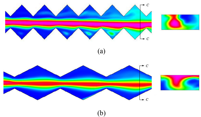
Fig. 6 Concentration distributions on the horizontal plane at z = 35\mu\text{m} of the flow in a micromixer with a grooved bottom, (a) \theta_c = 45^\circ and (b) \theta_c = 26^\circ 34' for the case with Re = 46.8
