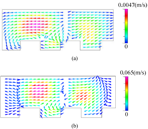
Fig. 4 Flow patterns on the vertical plane at x = 2000\mu\text{m} of the micromixer with grooved bottom and \theta_c = 45^\circ : (a) Re = 3 , (b) Re = 46.8
