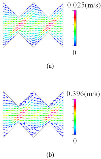
Fig. 3 Flow patterns on the horizontal plane at z = 5\mu\text{m} of the micromixer with grooved bottom and \theta_c = 45^\circ : (a) Re = 3 , (b) Re = 46.8
