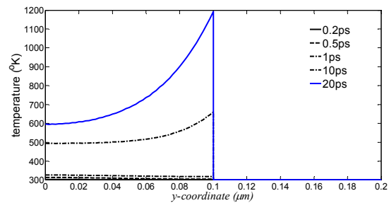
Fig. 10 Lattice temperature through thickness at x=5\mu\text{m} ( J=100\text{J}/\text{m}^2\text{K} )
