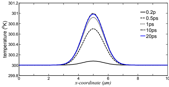
Fig. 8 Chromium's lattice temperature at y=0.1\mu\text{m} ( J=100\text{J}/\text{m}^2\text{K} )
