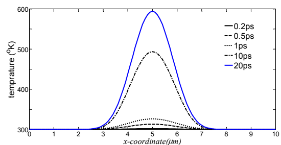
Fig. 6 Gold's lattice temperature at y=0.1\mu\text{m} ( J=100\text{J/m}^2\text{K} )
