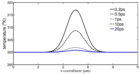
Fig. 7 Chromium's electron temperature at y=0.1\mu\text{m} ( J=100\text{J}/\text{m}^2\text{K} )
