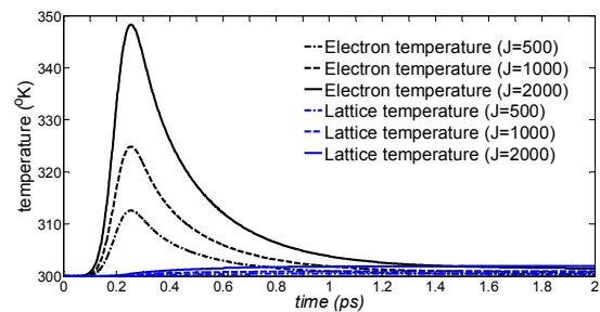
Fig. 4 Chromium's temperatures at x=5\mu\text{m}, y=0.1\mu\text{m}
