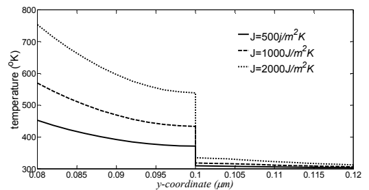
Fig. 11 Electron temperature through thickness at x=5\mu\text{m} , t=0.2\text{ps}
