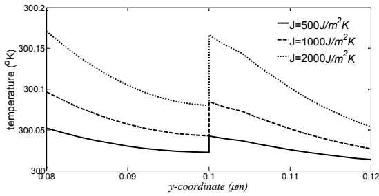
Fig. 12 Lattice temperature through thickness at x=5\mu\text{m} , t=0.2\text{ps}
