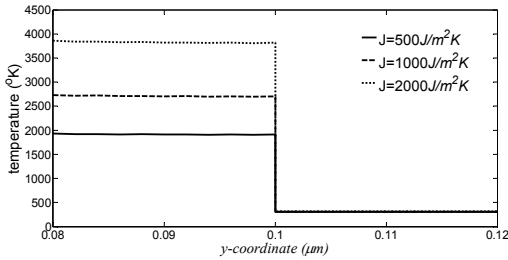
Fig. 13 Electron temperature through thickness at x=5\mu\text{m} , t=0.5\text{ps}
