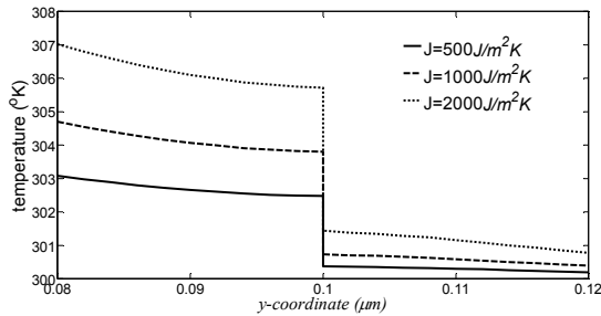
Fig. 14 Lattice temperature through thickness at x=5\mu\text{m} , t=0.5\text{ps}
