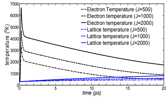
Fig. 3 Gold's temperatures at x=5\mu\text{m}, y=0\mu\text{m}
