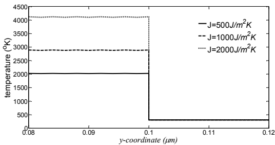
Fig. 15 Electron temperature through thickness at x=5\mu\text{m} , t=1\text{ps}
