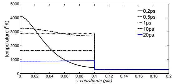
Fig. 9 Electron temperature through thickness at x=5\mu\text{m} ( J=100\text{J}/\text{m}^2\text{K} )
