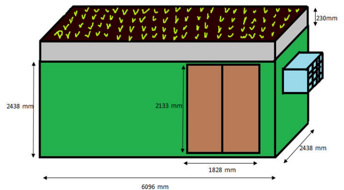
Fig. 2 Schematic diagram of experimental green roof [13]
