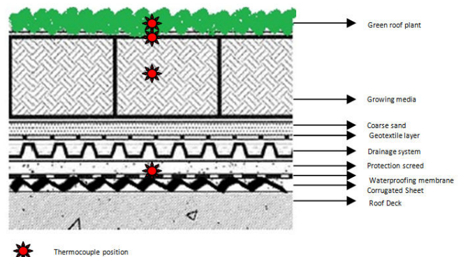
Fig. 4 An extensive green roof with different layers
