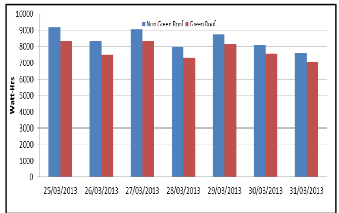
Fig. 10 Daily total energy consumption in March
