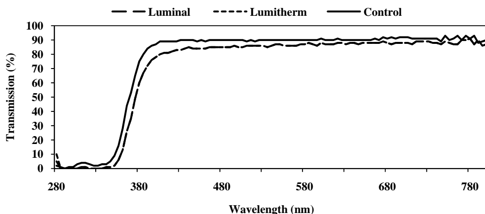
Fig. 1 Transmission spectra of each photosensitive film compared with control polythene film
