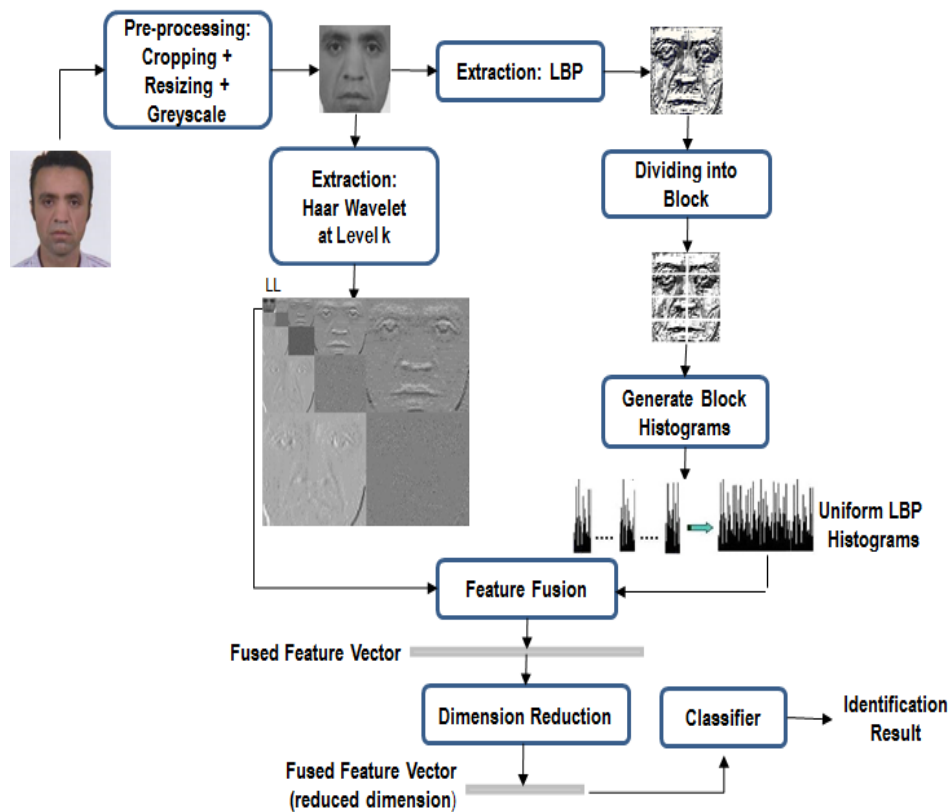
Fig. 4 The Framework of the Proposed Fusion Method
