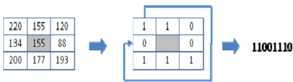
Fig. 1 Basic Local Binary Pattern Operation
