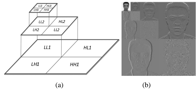
Fig. 2 Wavelet Transform (a) the pyramid scheme of resolutions; (b) an image transformed at level 3
