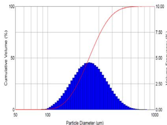
Fig.2 ZFS-JND particle size distribution of the coated
