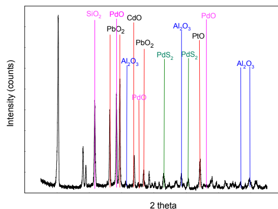
Fig. 4 HRXRD pattern of regenerated Pt-Pd catalyst
