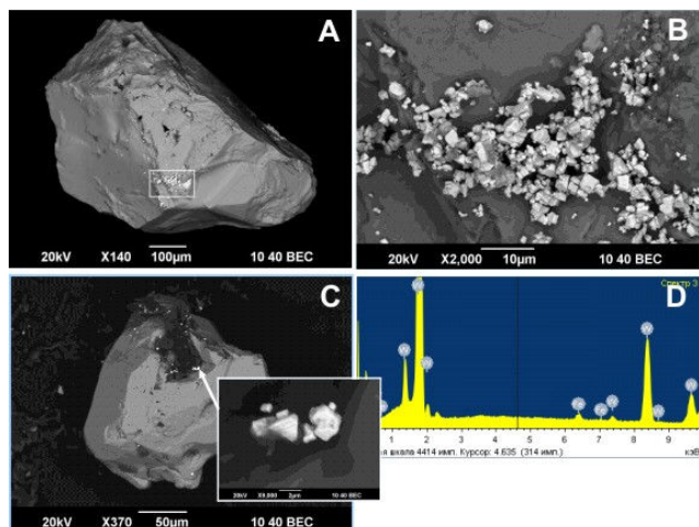
Fig. 4 Native tungsten on pyrite (Bogomol deposit) (A), (B) druse-like growths (C) native tungsten on the periphery of bitumen inclusions (dark area) (D) example of energy dispersive spectrum of one of the tungsten grains
