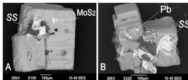
Fig. 3 Growths of Zn-containing grey copper ore (SS), inclusions of molybdenite (A) and native lead+anglesite? phases (B) on surfaces of pyrite grains, Gumeshki
