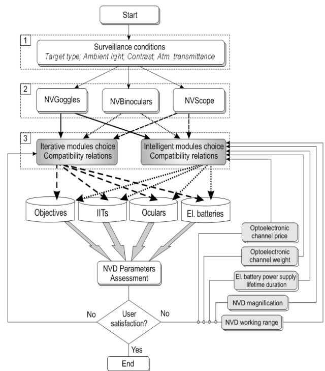
Fig. 2 Flowchart of the NVDs design algorithm
