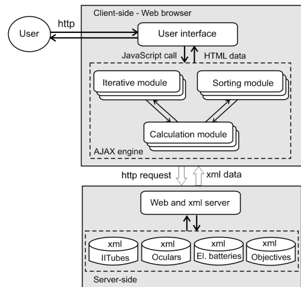
Fig. 3 Architecture of the intelligent Web-based system
