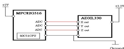
Fig. 1 Hardware architecture
