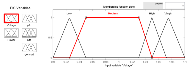
Fig. 4 Input voltage membership functions
