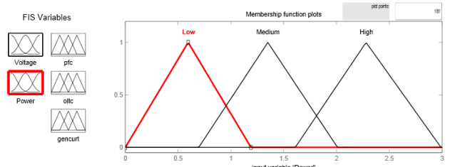
Fig. 5 DG input power membership functions
