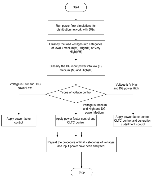
Fig. 3 Flowchart for fuzzy logic voltage control system
