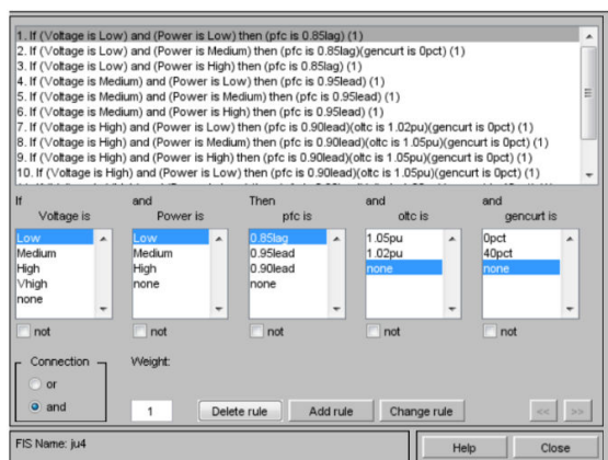
Fig. 9 Fuzzy Logic Control Rules
