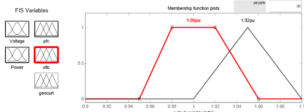
Fig.7 On Load Tap Changer (OLTC) membership functions
