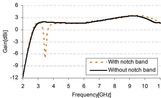
Fig. 6 Peak gain of the proposed antenna
