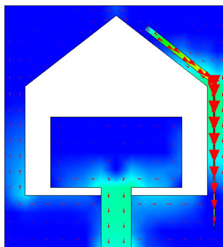
Fig. 2 Surface current distribution at 3.5 GHz
