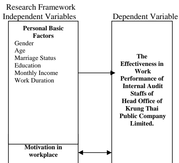
Fig. 1 Conceptual Framework
