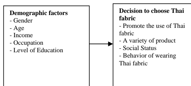
Fig. 1 Conceptual Framework
