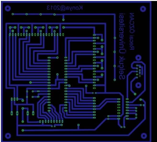
Fig. 1 PCB of designed system
