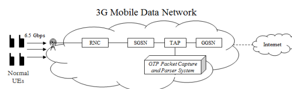
Fig. 3 The monitoring environment
