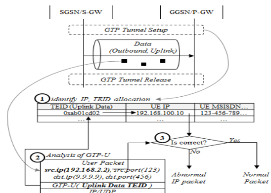
Fig. 7 Scheme for abnormal IP packets detection
