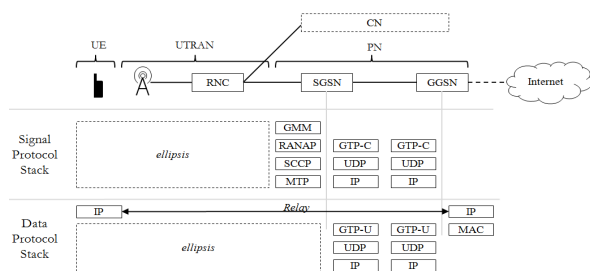
Fig. 1 3G mobile network structure
